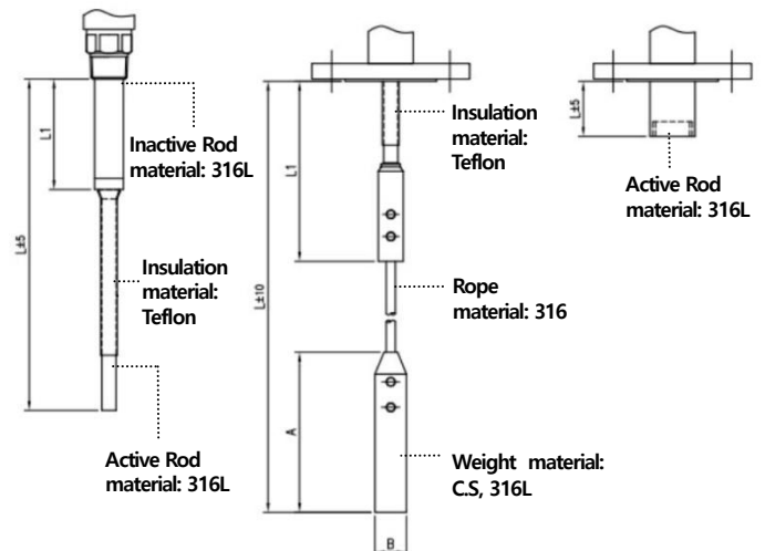
Rope Type
